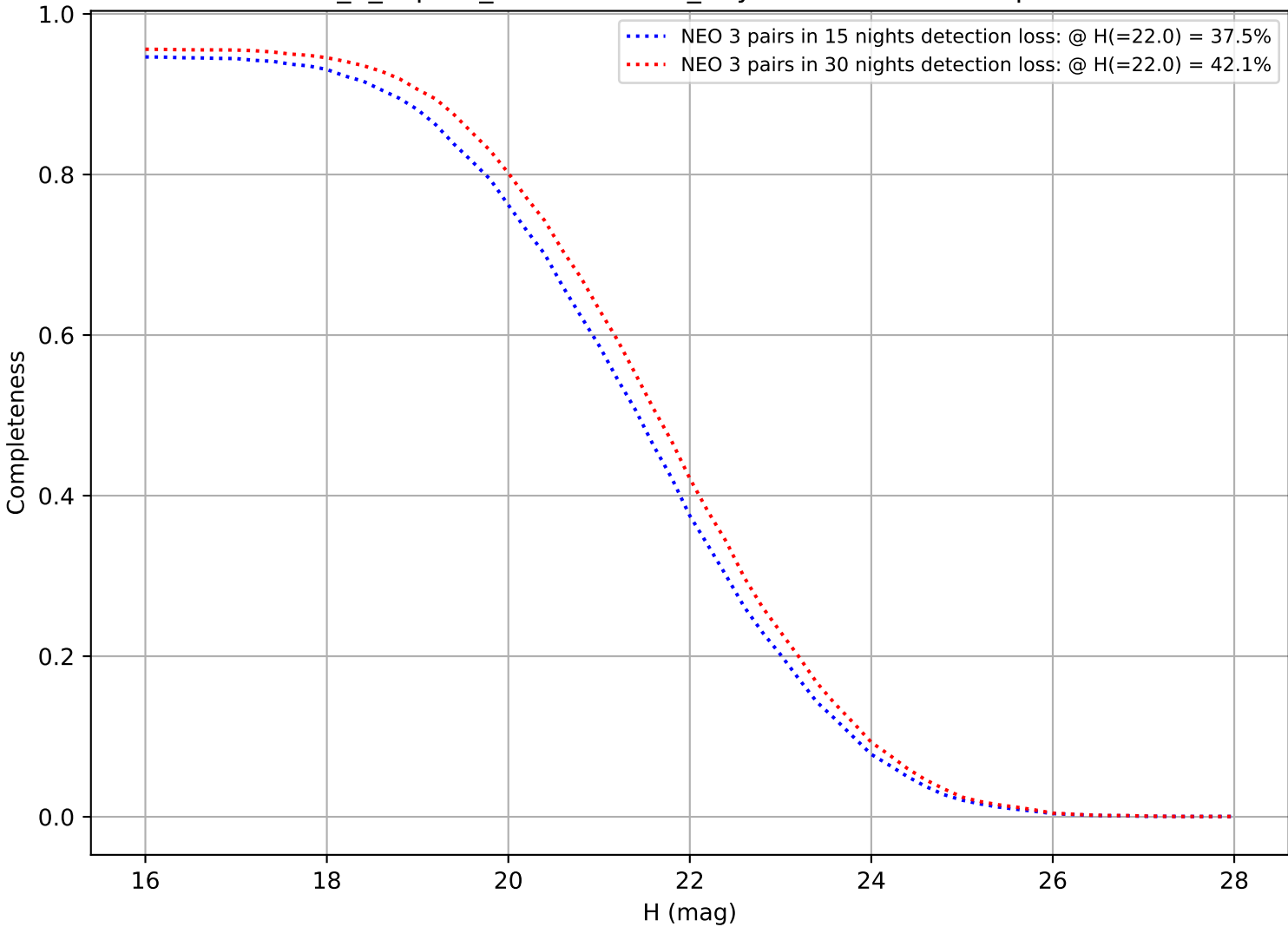
internal_u_expt38_nscale1.0v3.4_10yrs: DifferentialCompleteness
