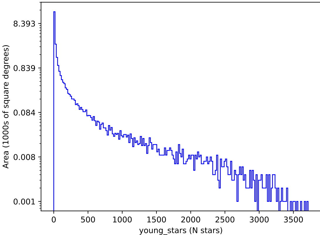
internal_u_expt38_nscale1.0v3.4_10yrs : young_stars
