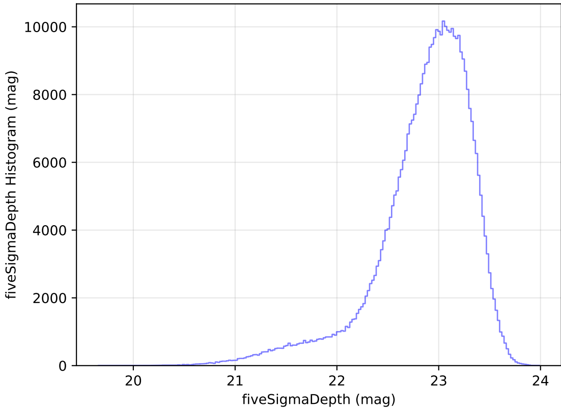
internal_u_expt38_nscale1.0v3.4_10yrs z: fiveSigmaDepth Histogram
