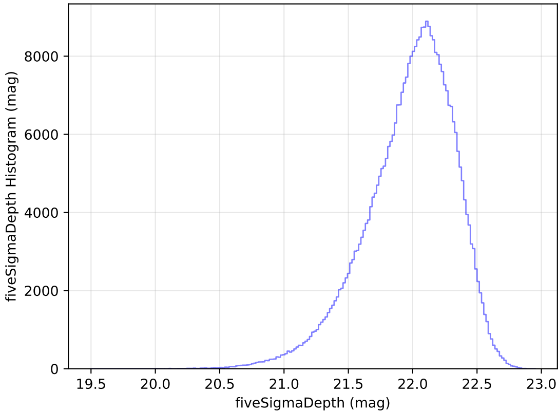
internal_u_expt38_nscale1.0v3.4_10yrs y: fiveSigmaDepth Histogram
