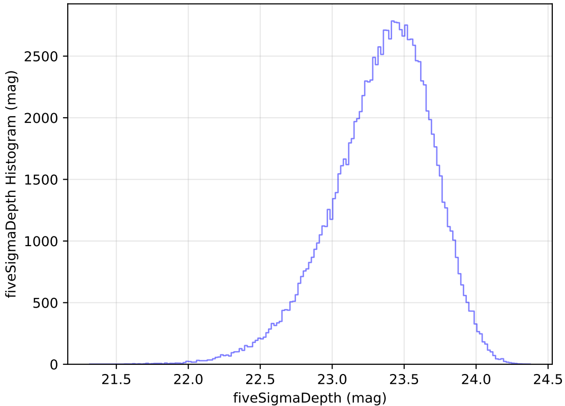
internal_u_expt38_nscale1.0v3.4_10yrs u: fiveSigmaDepth Histogram
