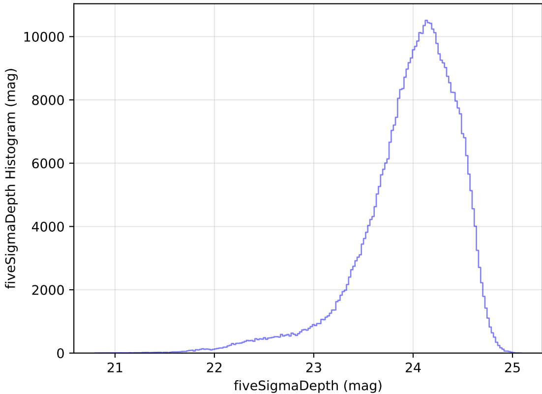
internal_u_expt38_nscale1.0v3.4_10yrs r: fiveSigmaDepth Histogram
