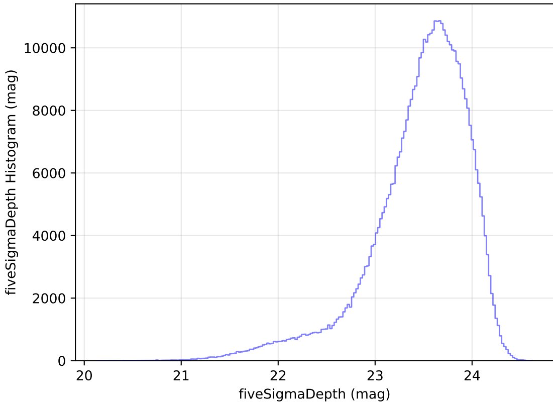
internal_u_expt38_nscale1.0v3.4_10yrs i: fiveSigmaDepth Histogram
