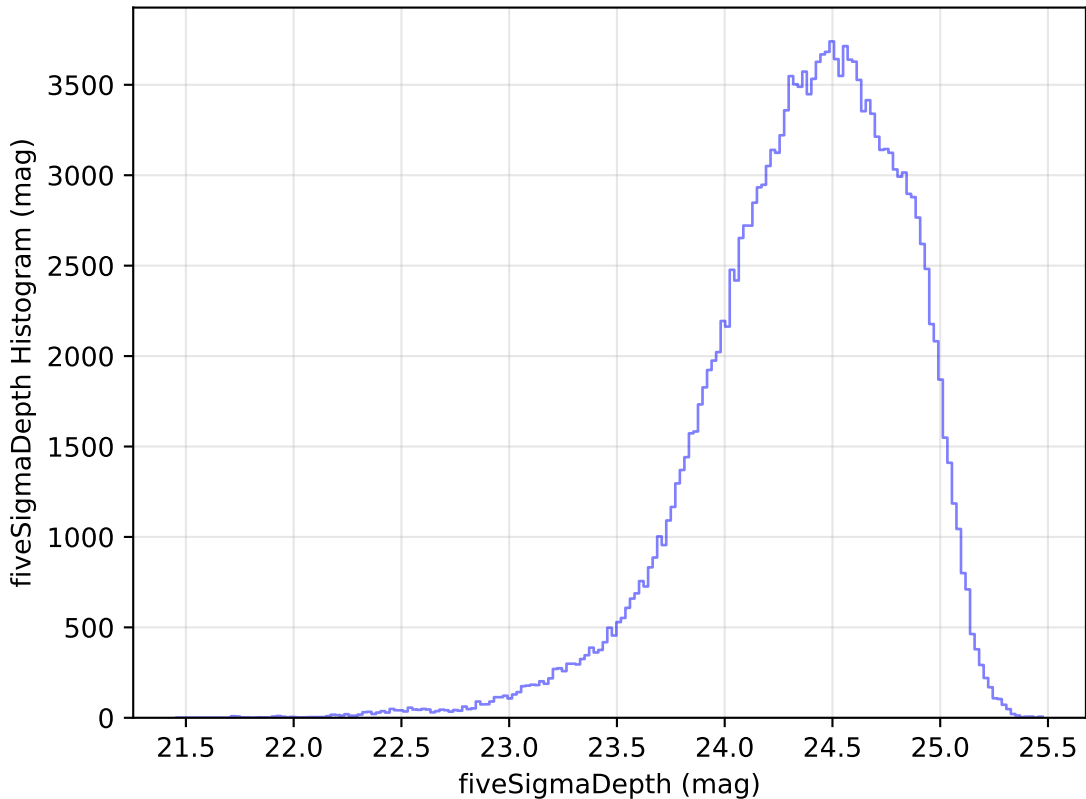
internal_u_expt38_nscale1.0v3.4_10yrs g: fiveSigmaDepth Histogram
