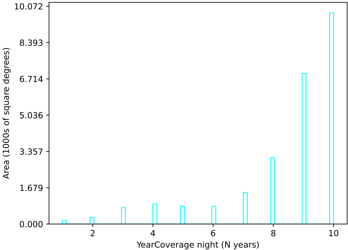
internal_u_expt38_nscale1.0v3.4_10yrs u band: YearCoverage night
