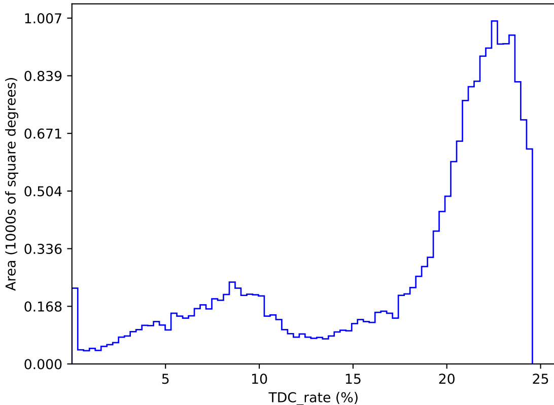
internal_u_expt38_nscale1.0v3.4_10yrs : TDC_rate
