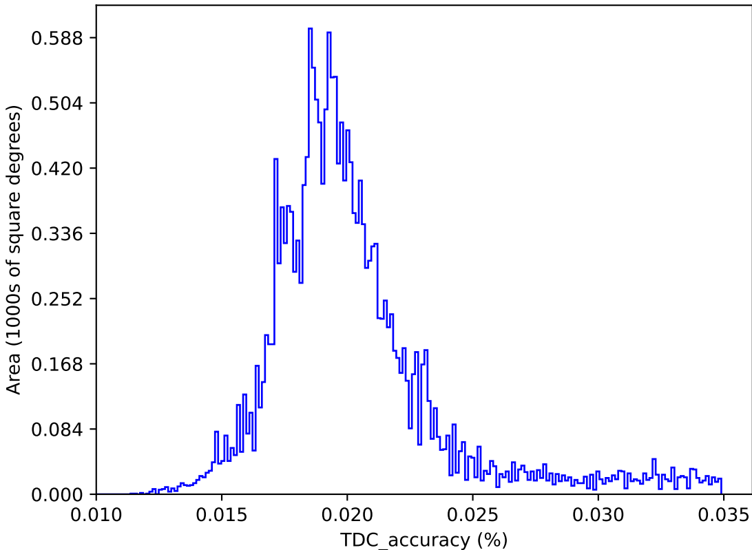
internal_u_expt38_nscale1.0v3.4_10yrs : TDC_accuracy
