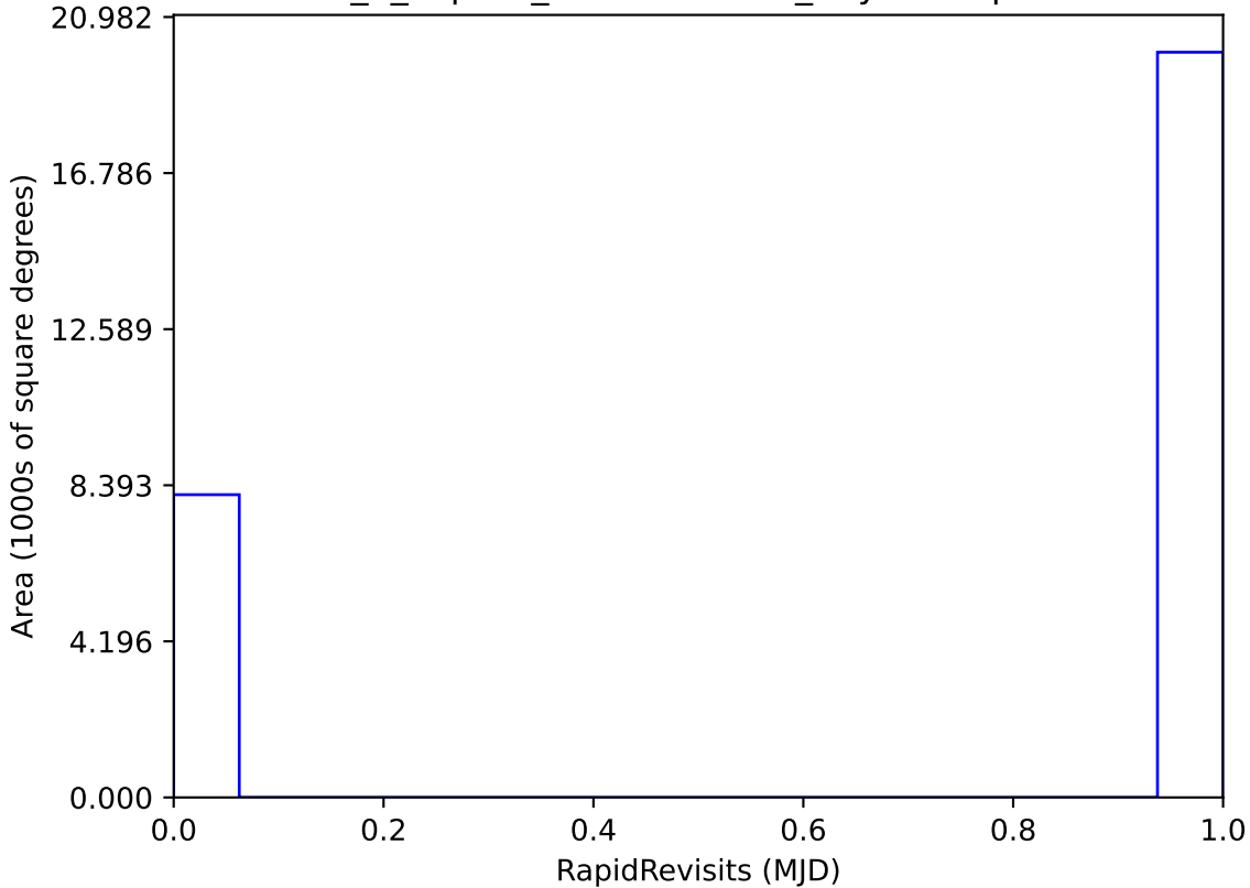
internal_u_expt38_nscale1.0v3.4_10yrs : RapidRevisits
