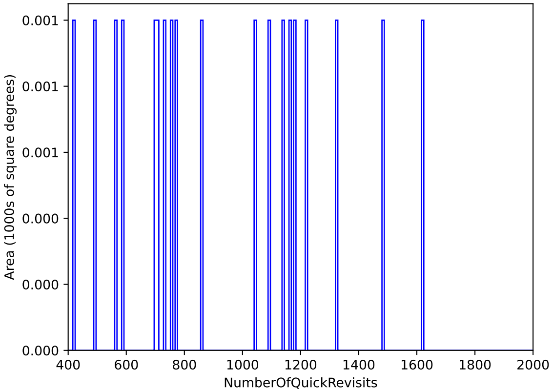
internal_u_expt38_nscale1.0v3.4_10yrs : NumberOfQuickRevisits
