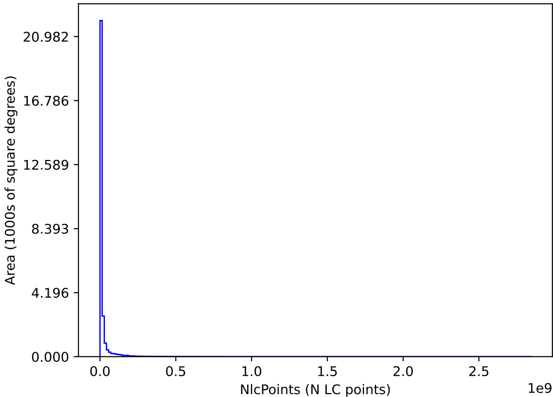
internal_u_expt38_nscale1.0v3.4_10yrs : NlcPoints
