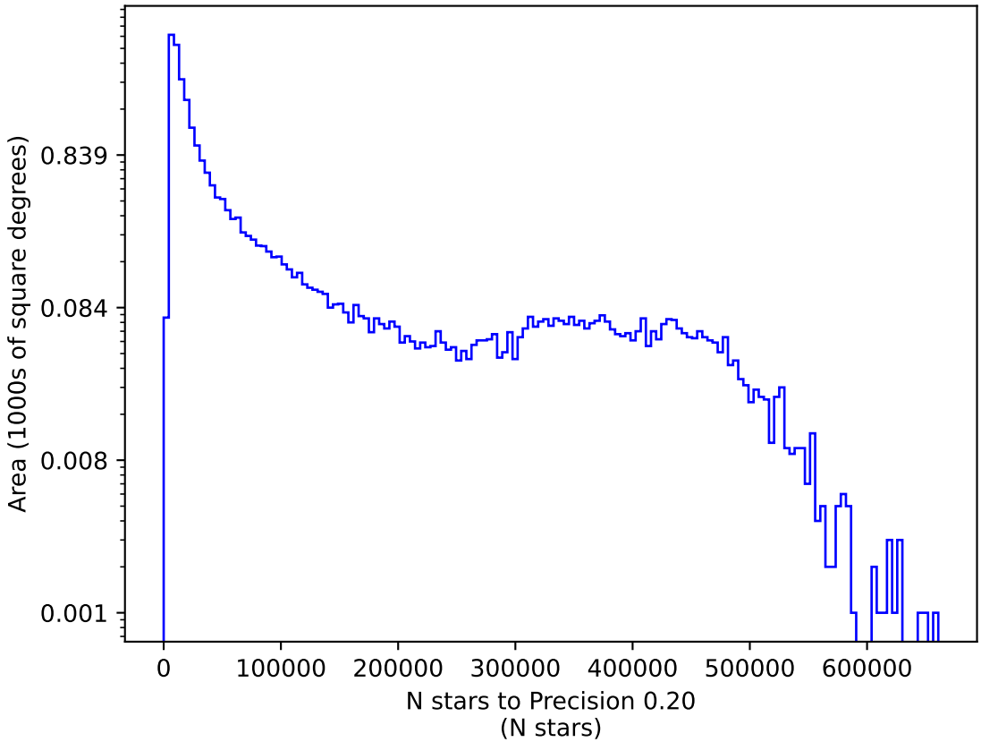
internal_u_expt38_nscale1.0v3.4_10yrs r: N stars to Precision 0.20
