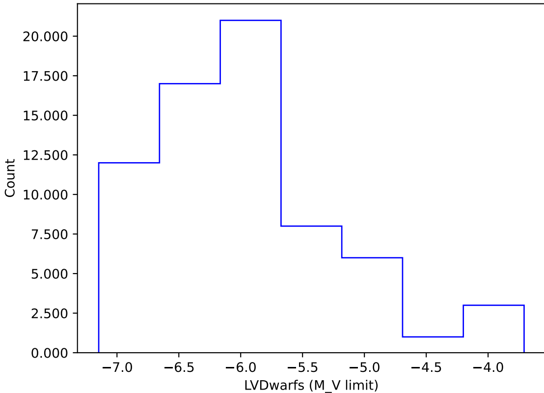
internal_u_expt38_nscale1.0v3.4_10yrs gi: LVDwarfs
