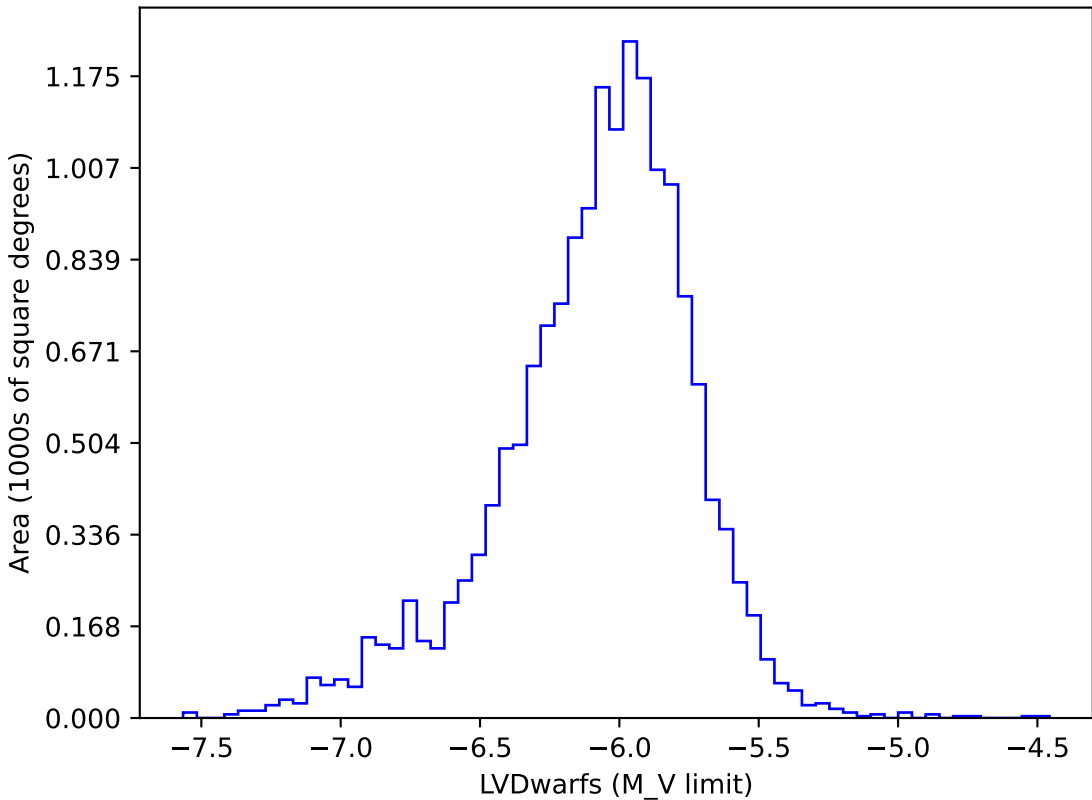
internal_u_expt38_nscale1.0v3.4_10yrs gi: LVDwarfs
