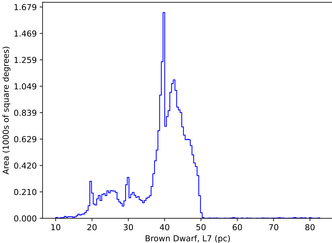
internal_u_expt38_nscale1.0v3.4_10yrs : Brown Dwarf, L7
