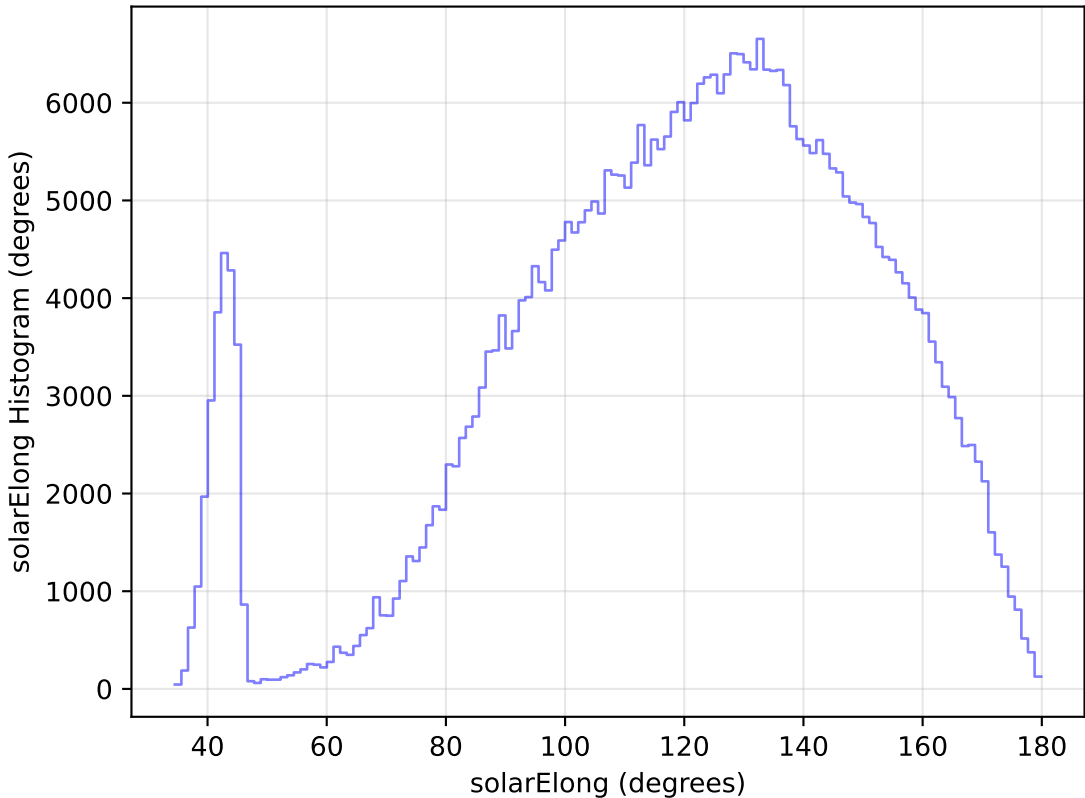
internal_u_expt38_nscale1.0v3.4_10yrs WFD z band: solarElong Histogram
