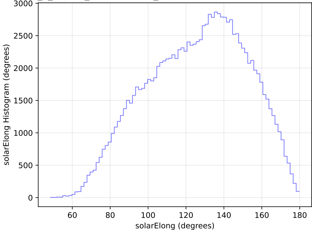
internal_u_expt38_nscale1.0v3.4_10yrs WFD u band: solarElong Histogram
