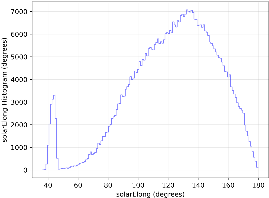
internal_u_expt38_nscale1.0v3.4_10yrs WFD r band: solarElong Histogram
