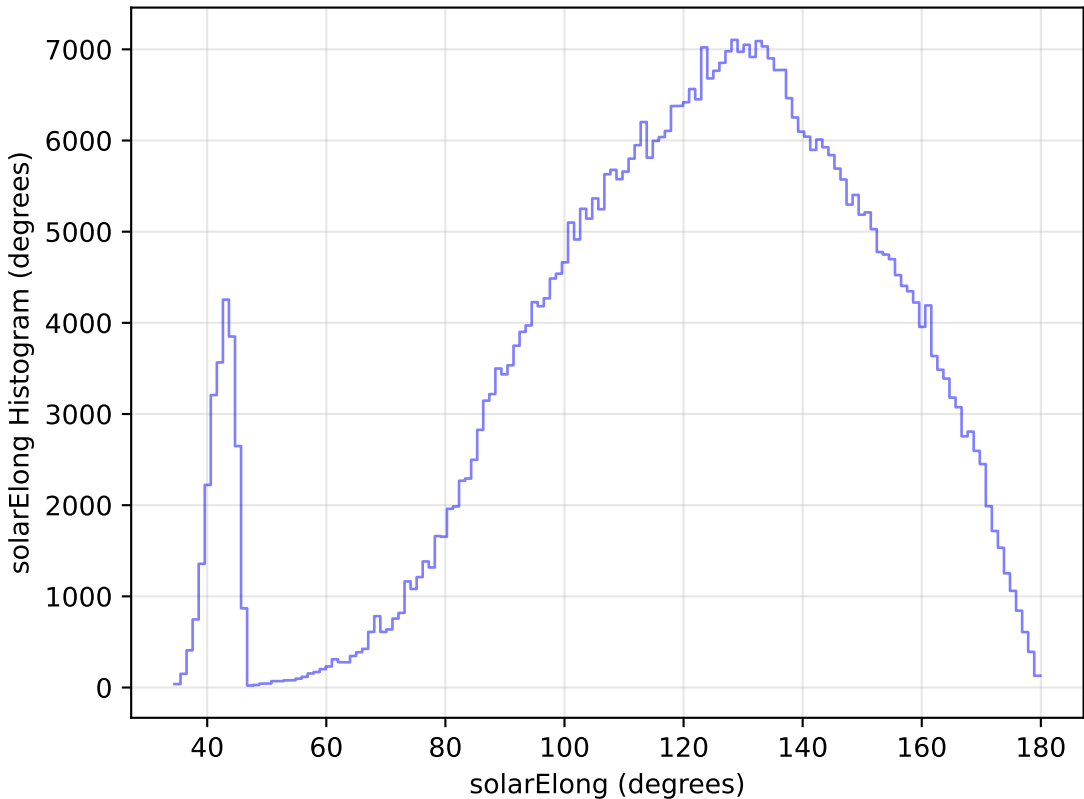
internal_u_expt38_nscale1.0v3.4_10yrs WFD i band: solarElong Histogram
