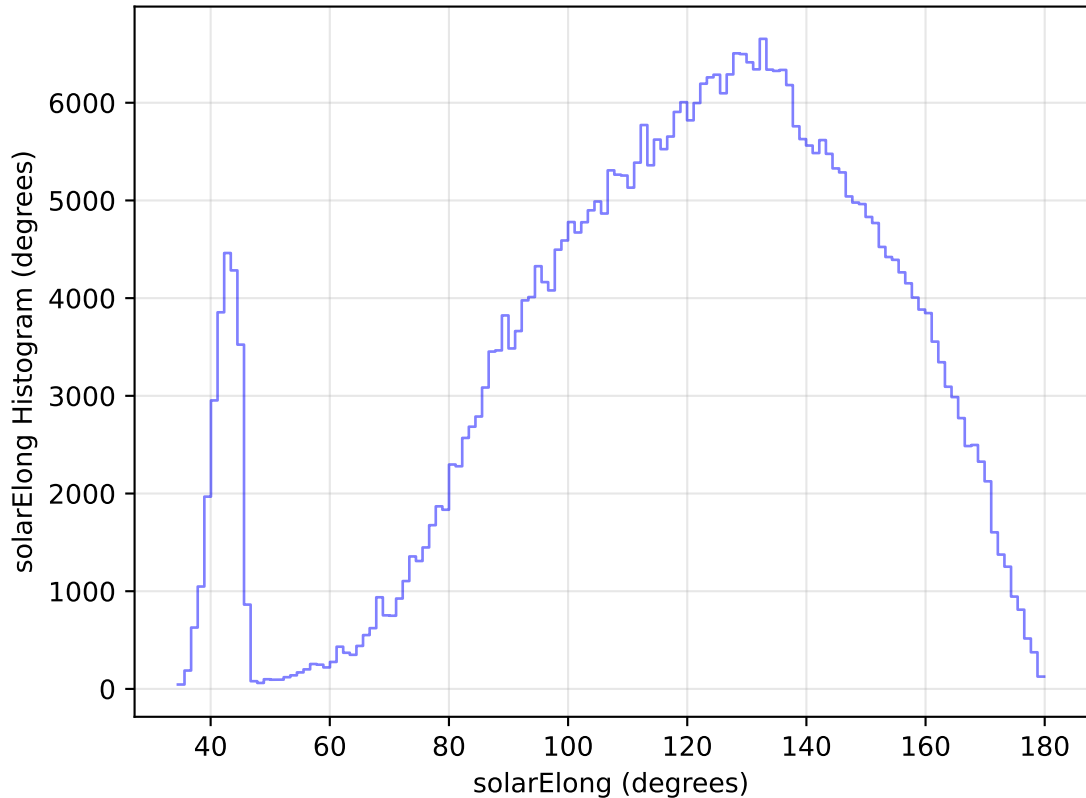
internal_u_expt38_nscale1.0v3.4_10yrs All sky z band: solarElong Histogram
