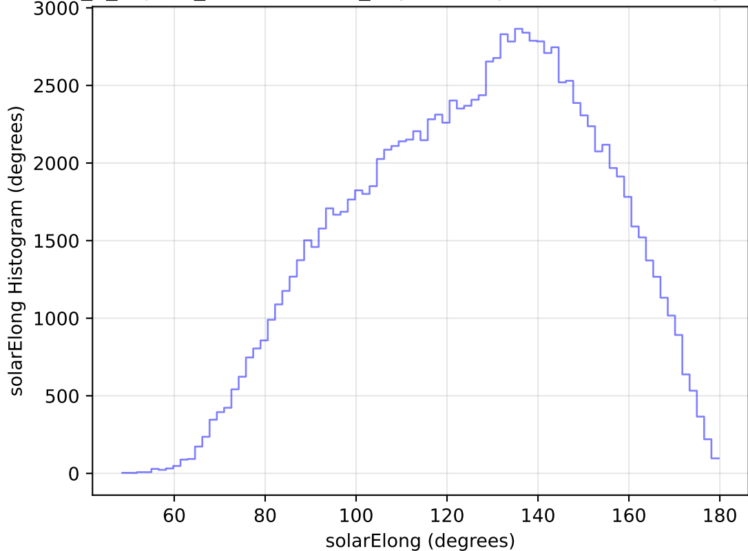
internal_u_expt38_nscale1.0v3.4_10yrs All sky u band: solarElong Histogram
