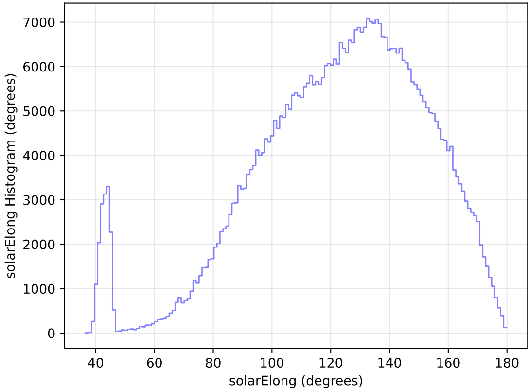
internal_u_expt38_nscale1.0v3.4_10yrs All sky r band: solarElong Histogram
