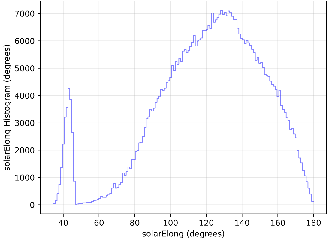
internal_u_expt38_nscale1.0v3.4_10yrs All sky i band: solarElong Histogram
