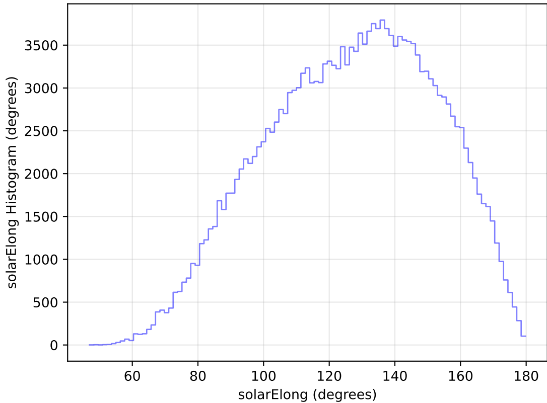
internal_u_expt38_nscale1.0v3.4_10yrs All sky g band: solarElong Histogram
