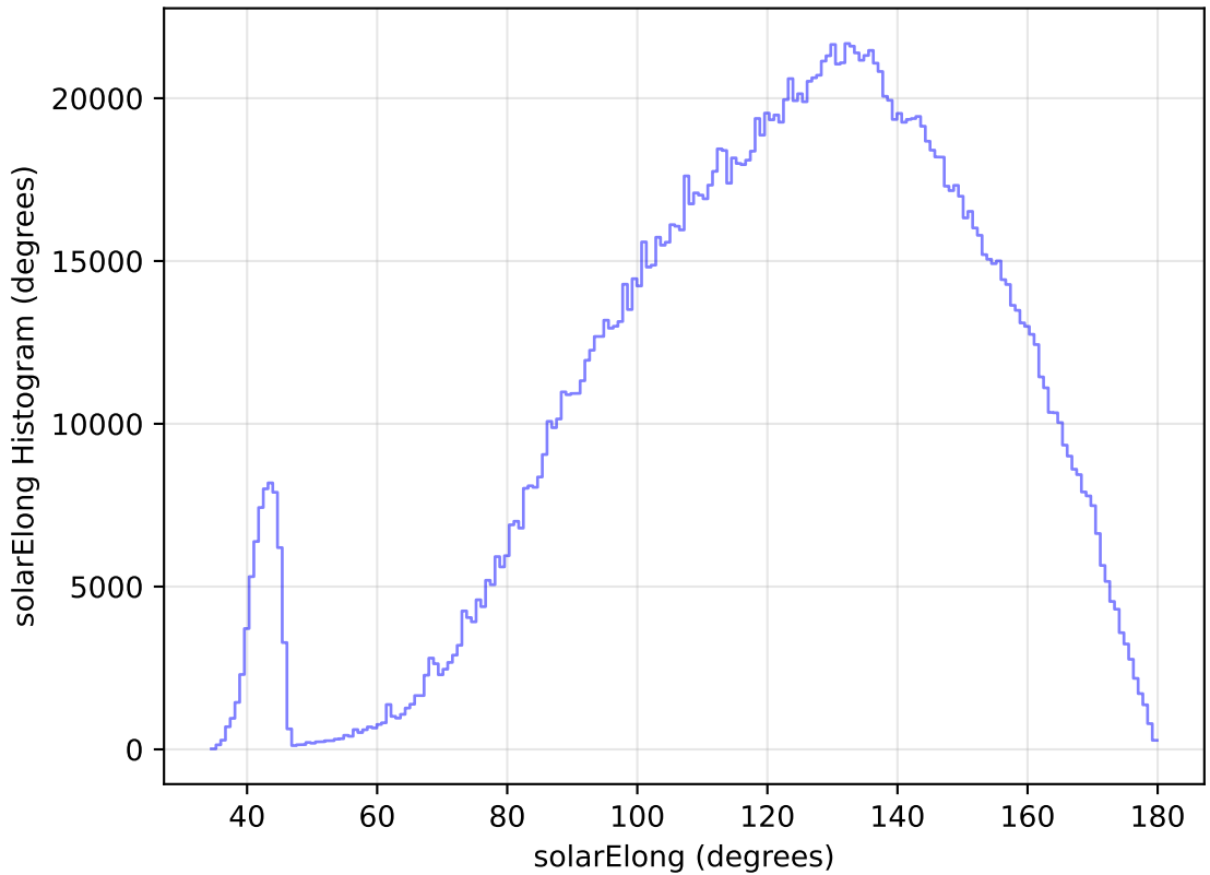
internal_u_expt38_nscale1.0v3.4_10yrs All sky all bands: solarElong Histogram
