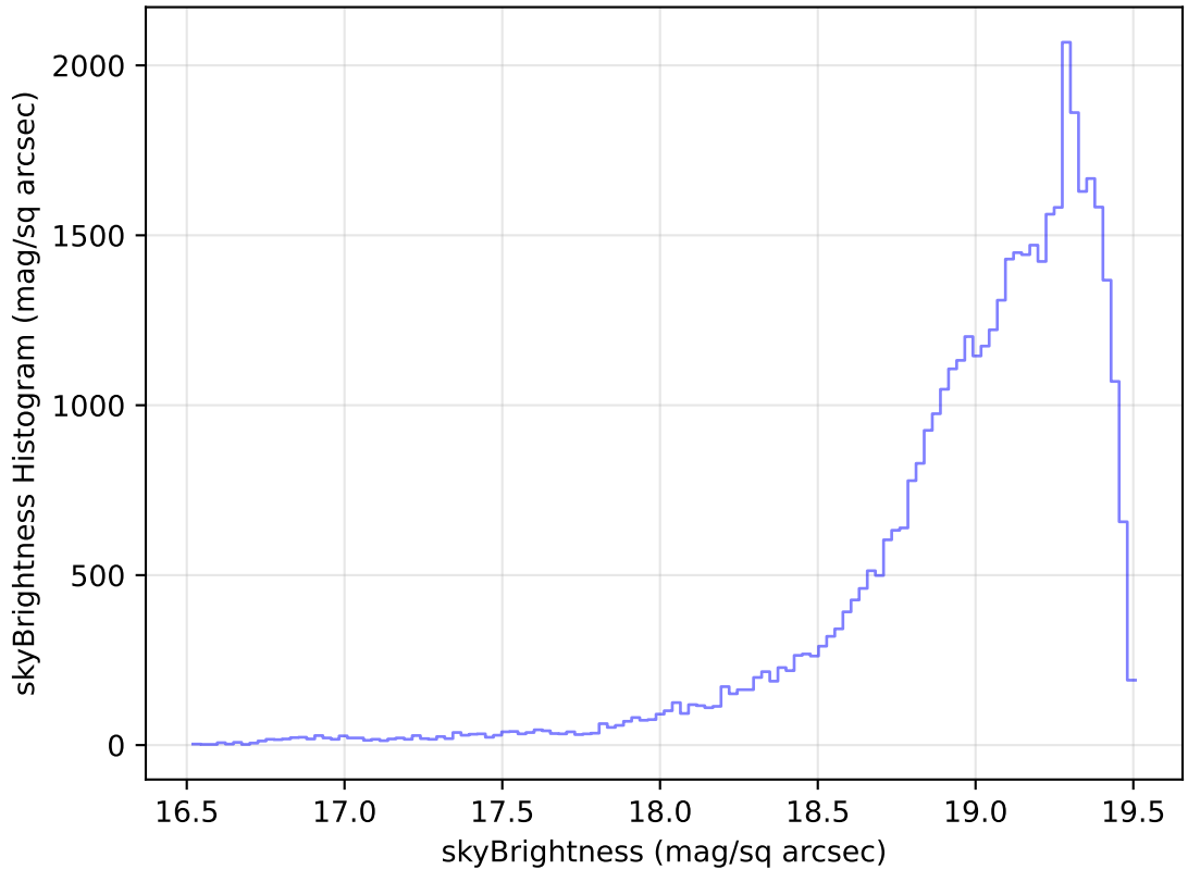
internal_u_expt38_nscale1.0v3.4_10yrs Yr 1 z band: skyBrightness Histogram
