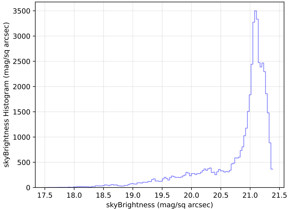
internal_u_expt38_nscale1.0v3.4_10yrs Yr 1 r band: skyBrightness Histogram
