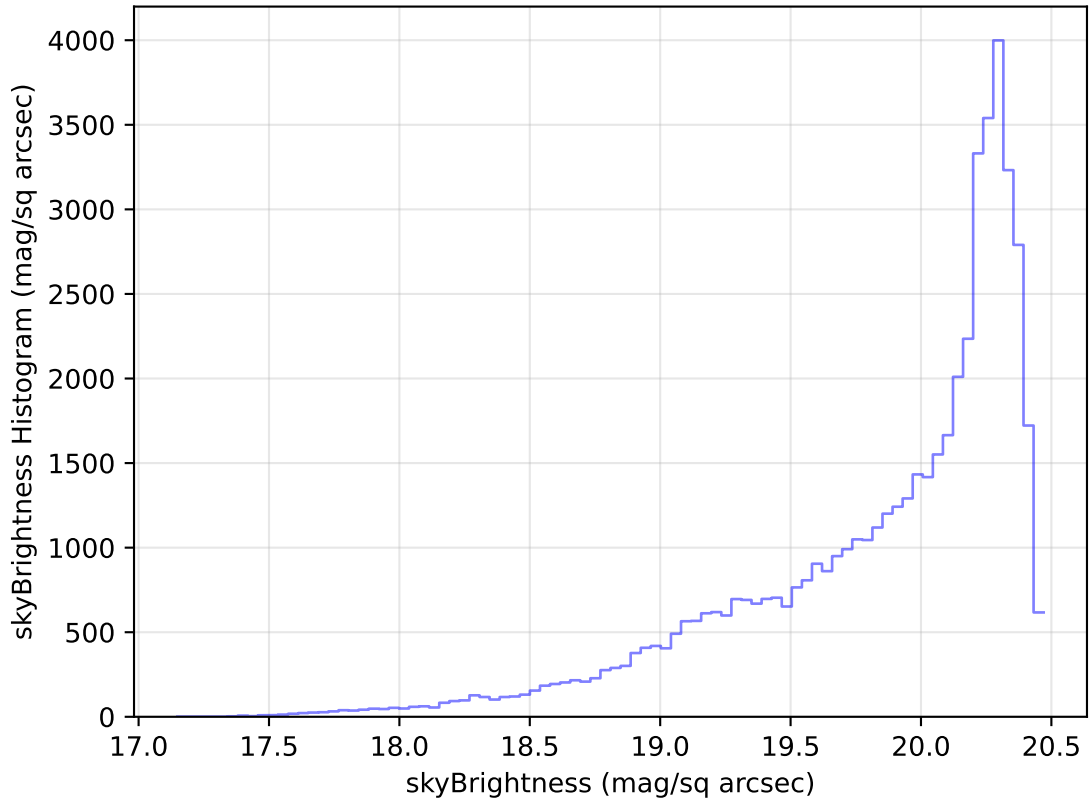
internal_u_expt38_nscale1.0v3.4_10yrs Yr 1 i band: skyBrightness Histogram
