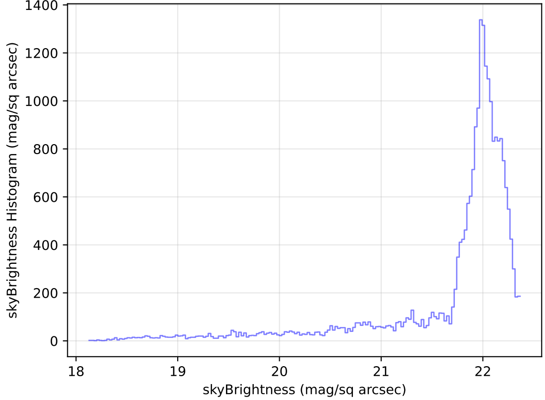
internal_u_expt38_nscale1.0v3.4_10yrs Yr 1 g band: skyBrightness Histogram
