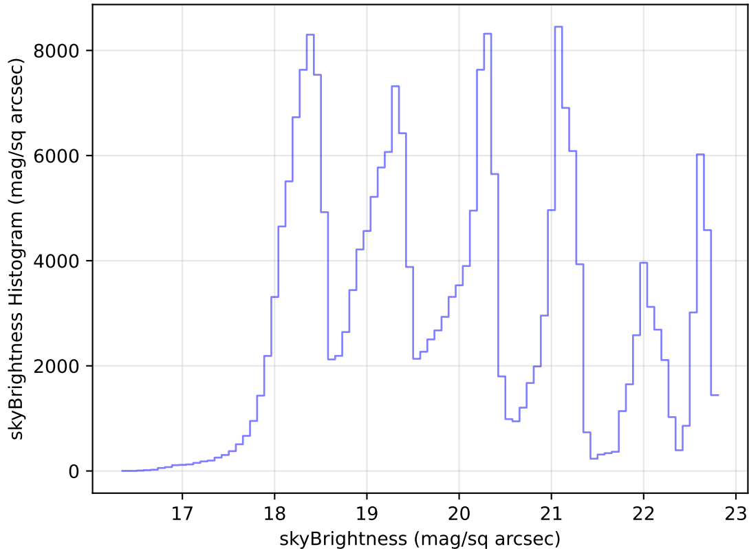
internal_u_expt38_nscale1.0v3.4_10yrs Yr 1 all bands: skyBrightness Histogram
