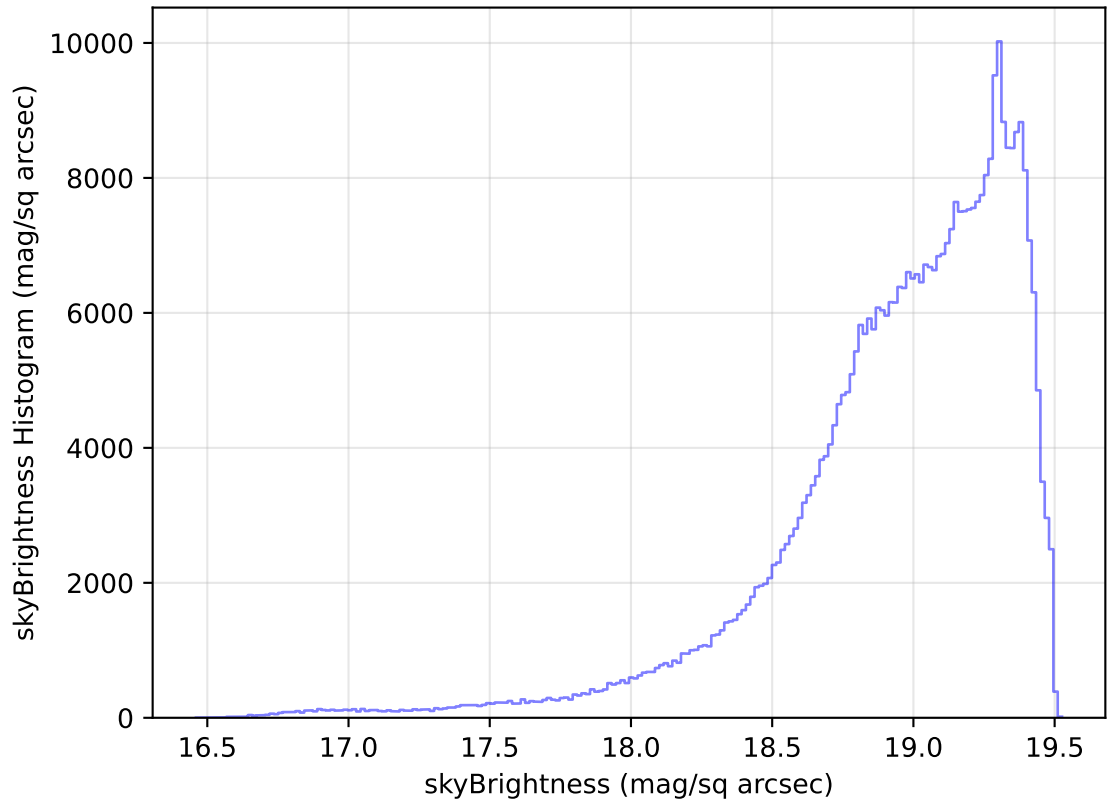
internal_u_expt38_nscale1.0v3.4_10yrs WFD z band: skyBrightness Histogram
