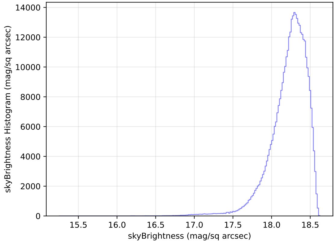
internal_u_expt38_nscale1.0v3.4_10yrs WFD y band: skyBrightness Histogram
