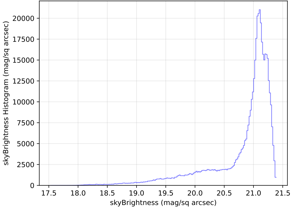
internal_u_expt38_nscale1.0v3.4_10yrs WFD r band: skyBrightness Histogram
