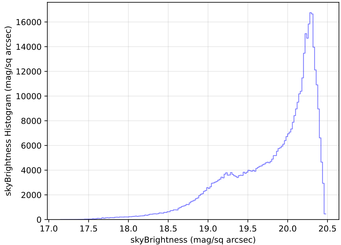
internal_u_expt38_nscale1.0v3.4_10yrs WFD i band: skyBrightness Histogram
