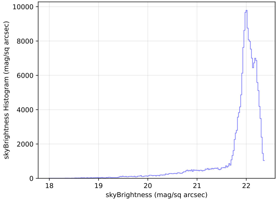
internal_u_expt38_nscale1.0v3.4_10yrs WFD g band: skyBrightness Histogram
