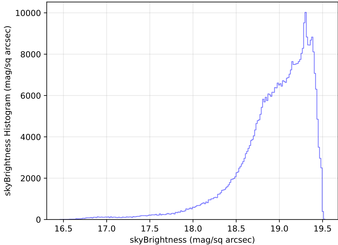
internal_u_expt38_nscale1.0v3.4_10yrs All sky z band: skyBrightness Histogram
