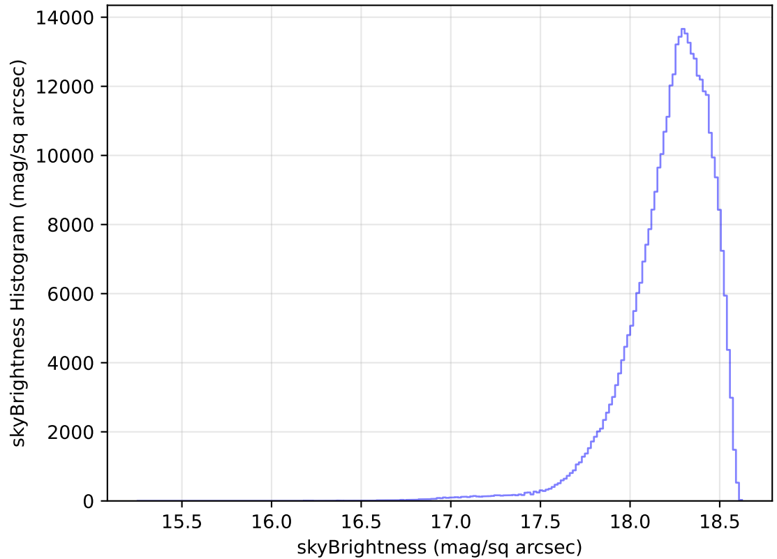
internal_u_expt38_nscale1.0v3.4_10yrs All sky y band: skyBrightness Histogram
