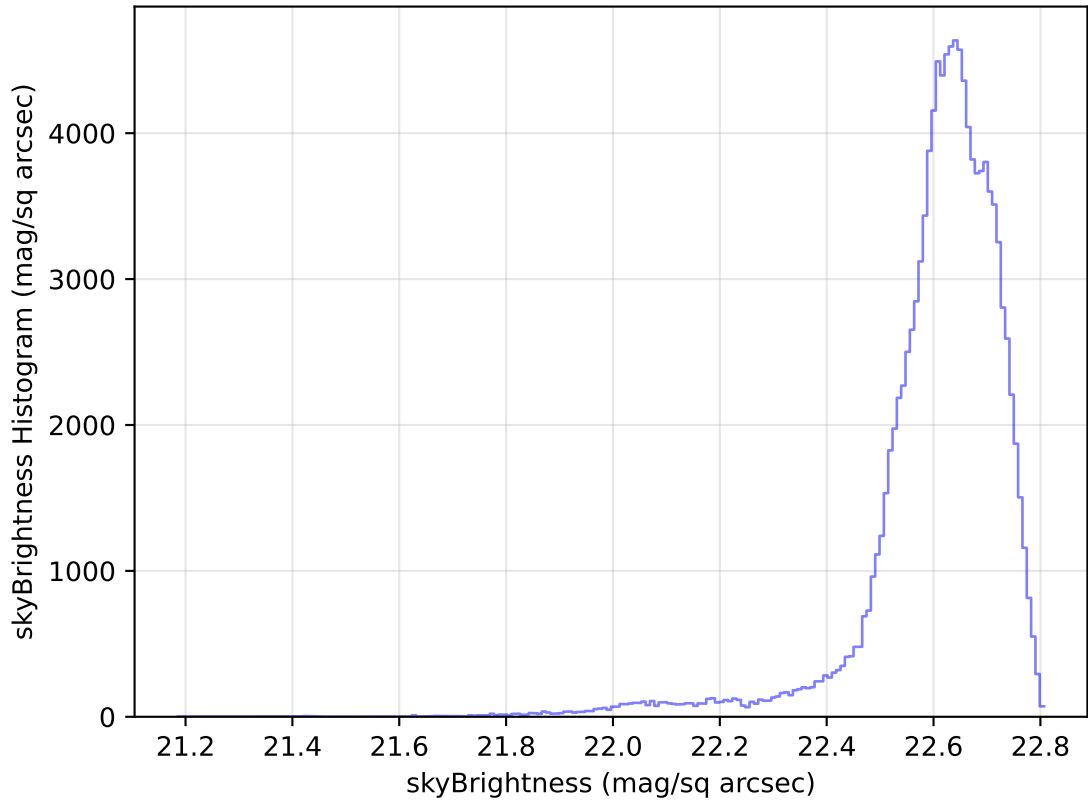
internal_u_expt38_nscale1.0v3.4_10yrs All sky u band: skyBrightness Histogram
