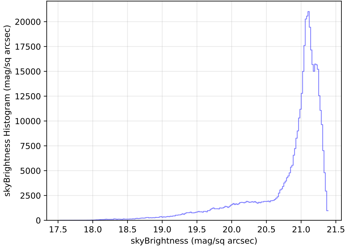
internal_u_expt38_nscale1.0v3.4_10yrs All sky r band: skyBrightness Histogram
