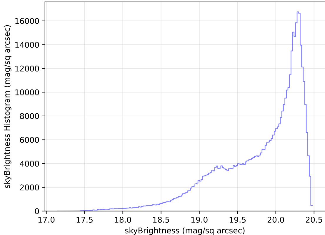
internal_u_expt38_nscale1.0v3.4_10yrs All sky i band: skyBrightness Histogram
