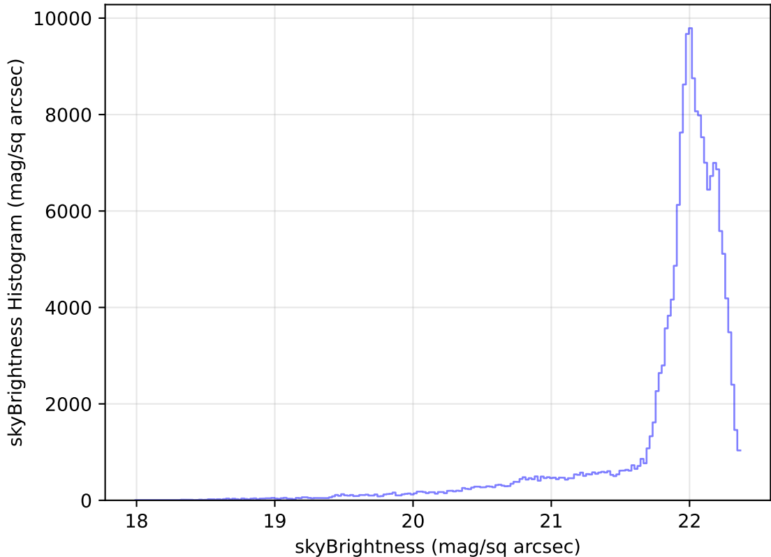
internal_u_expt38_nscale1.0v3.4_10yrs All sky g band: skyBrightness Histogram
