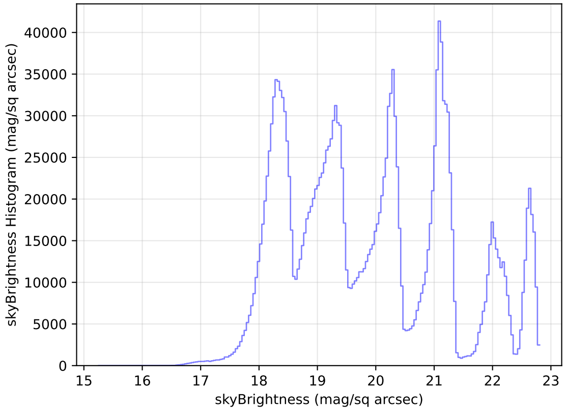
internal_u_expt38_nscale1.0v3.4_10yrs All sky all bands: skyBrightness Histogram
