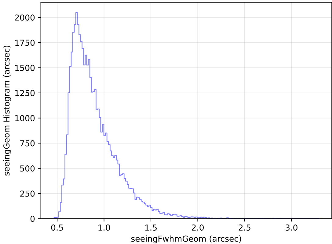
internal_u_expt38_nscale1.0v3.4_10yrs Yr 1 r band: seeingGeom Histogram
