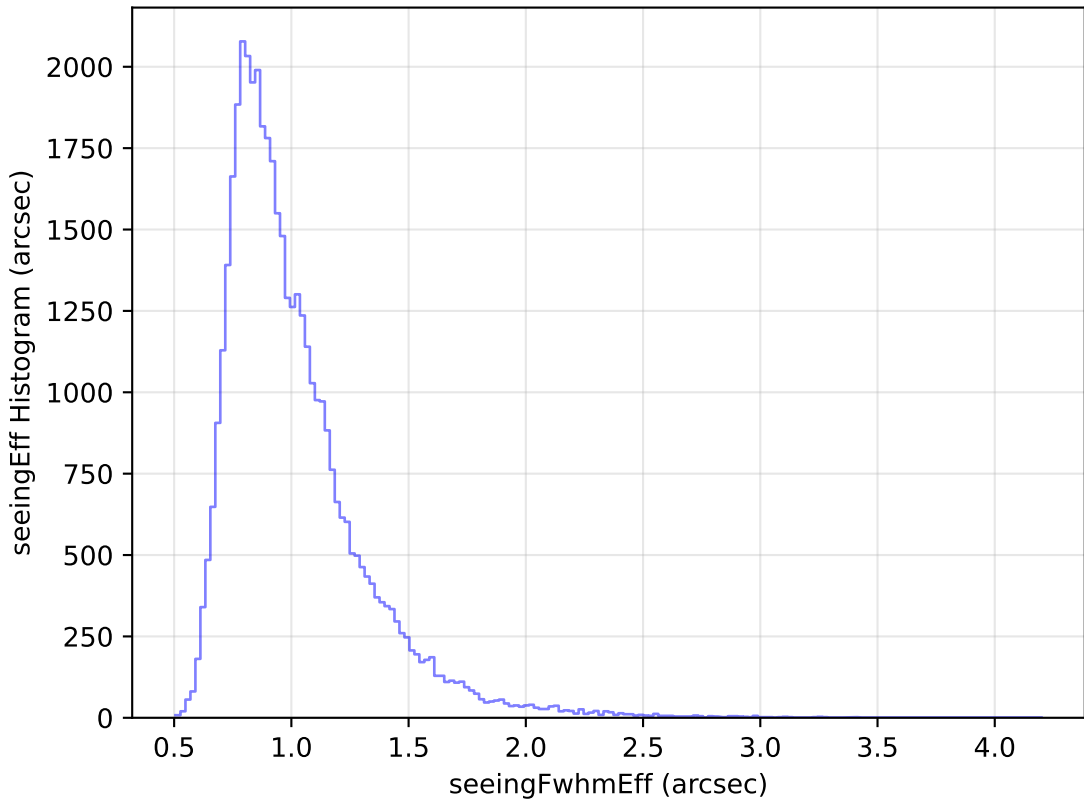
internal_u_expt38_nscale1.0v3.4_10yrs Yr 1 z band: seeingEff Histogram
