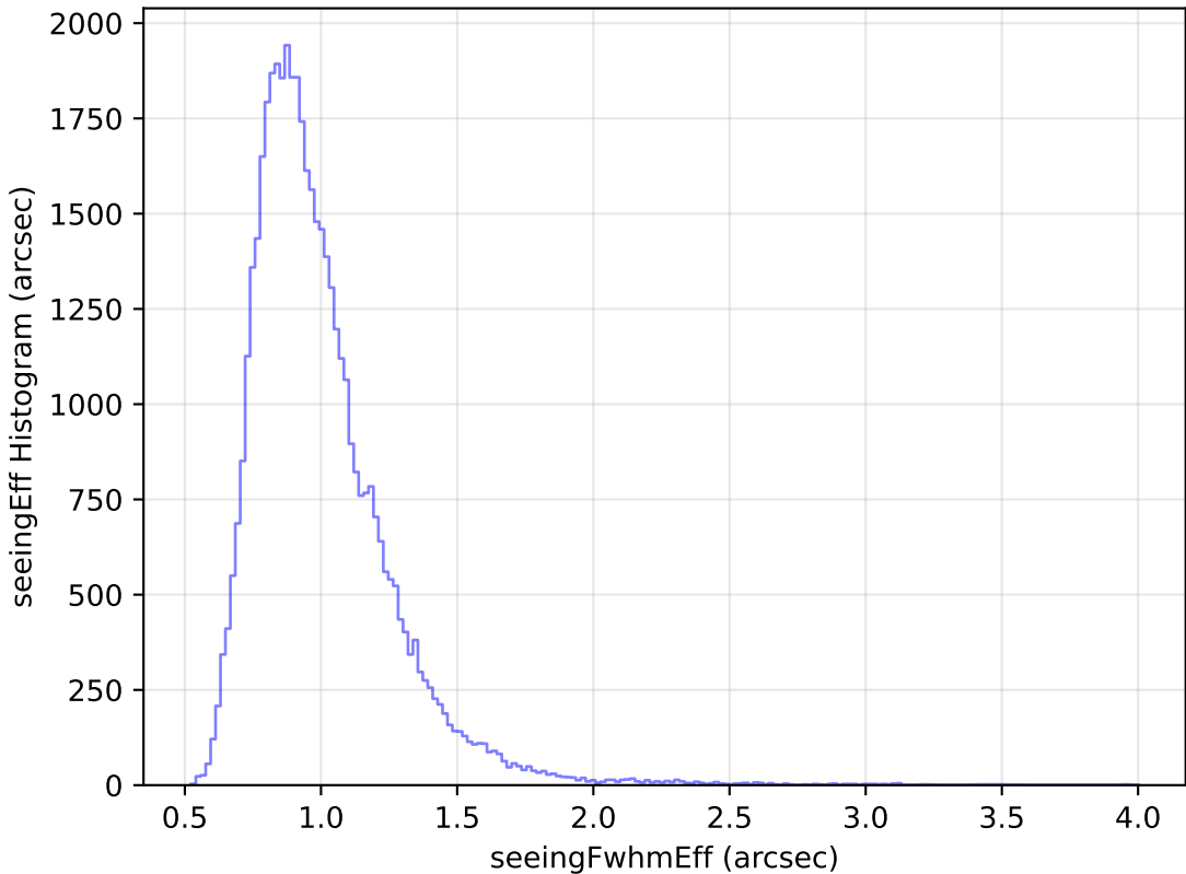
internal_u_expt38_nscale1.0v3.4_10yrs Yr 1 y band: seeingEff Histogram
