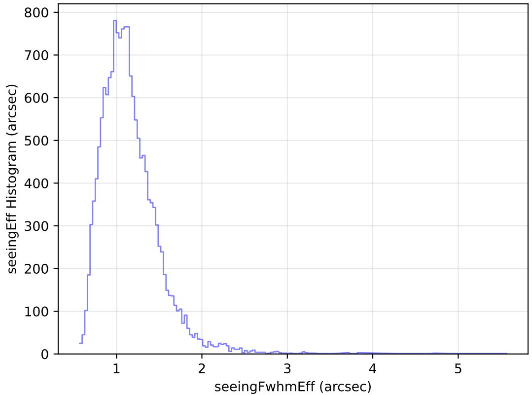
internal_u_expt38_nscale1.0v3.4_10yrs Yr 1 u band: seeingEff Histogram
