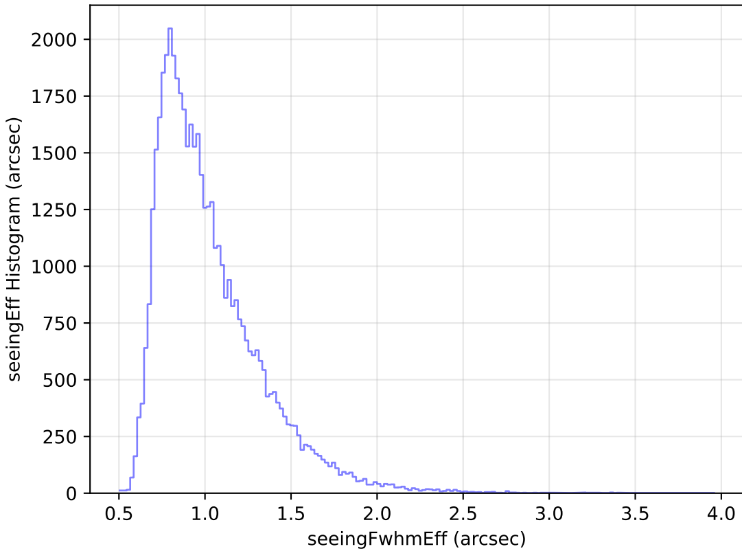
internal_u_expt38_nscale1.0v3.4_10yrs Yr 1 r band: seeingEff Histogram
